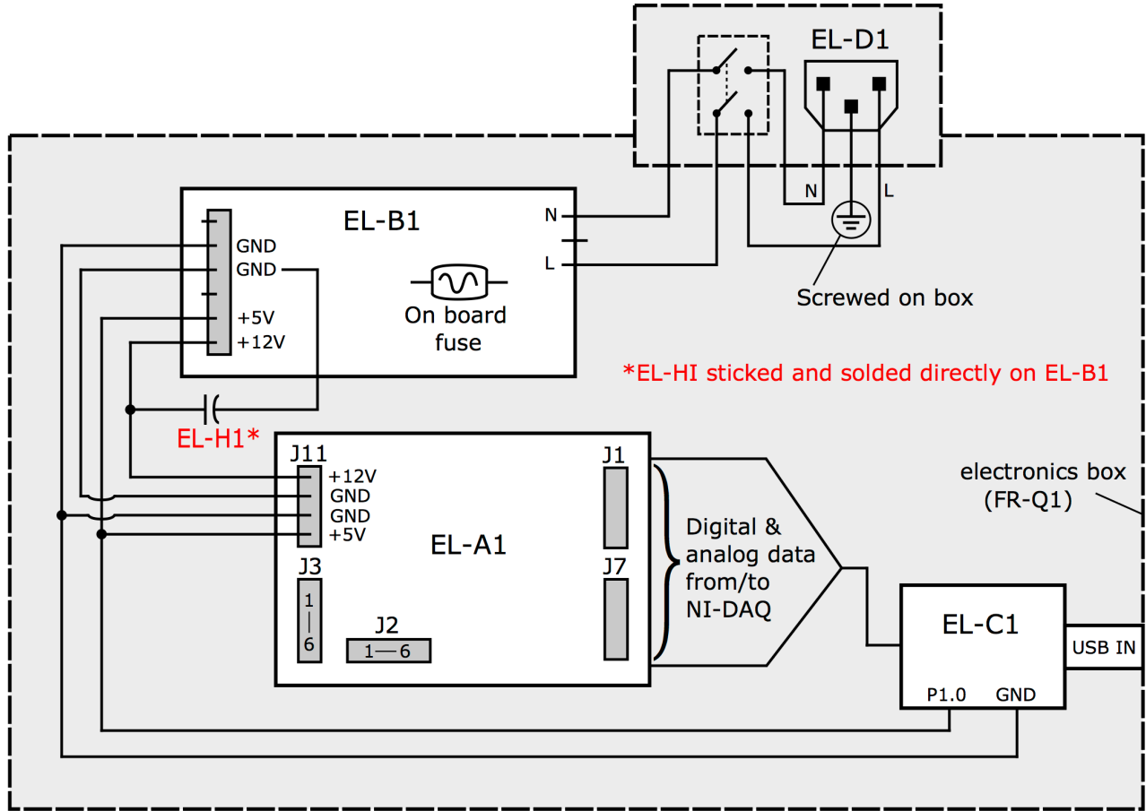
Figure 4 - Assembly of the main electronics components (Figure S4)
