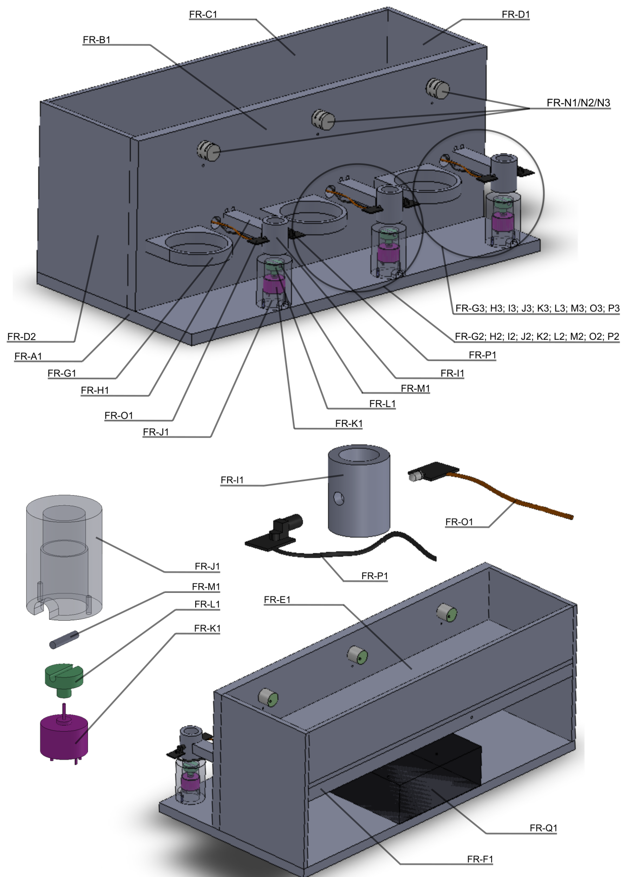
Figure 1 - Frame assembly (Figure S1)
