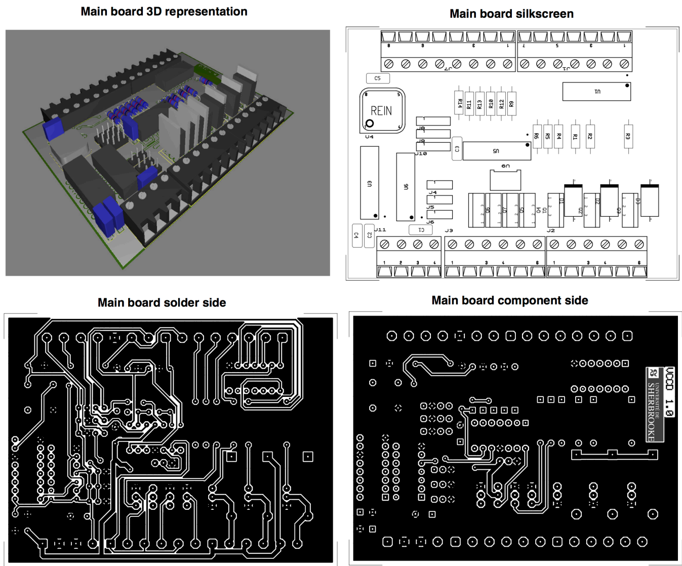
Figure 7 - Details of the main PCB (Figure S7)
