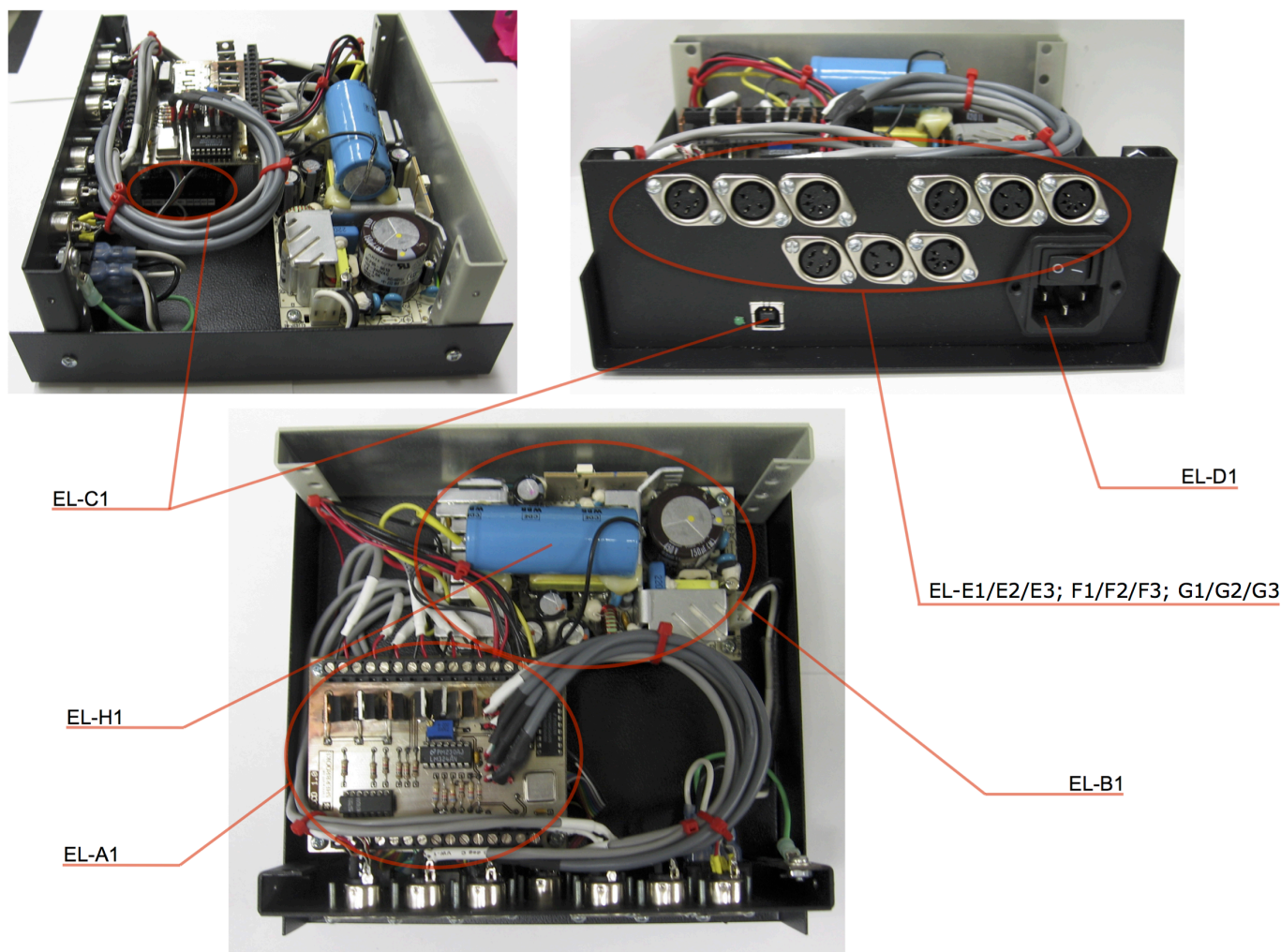
Figure 3 - Electronics box assembly (Figure S3)
