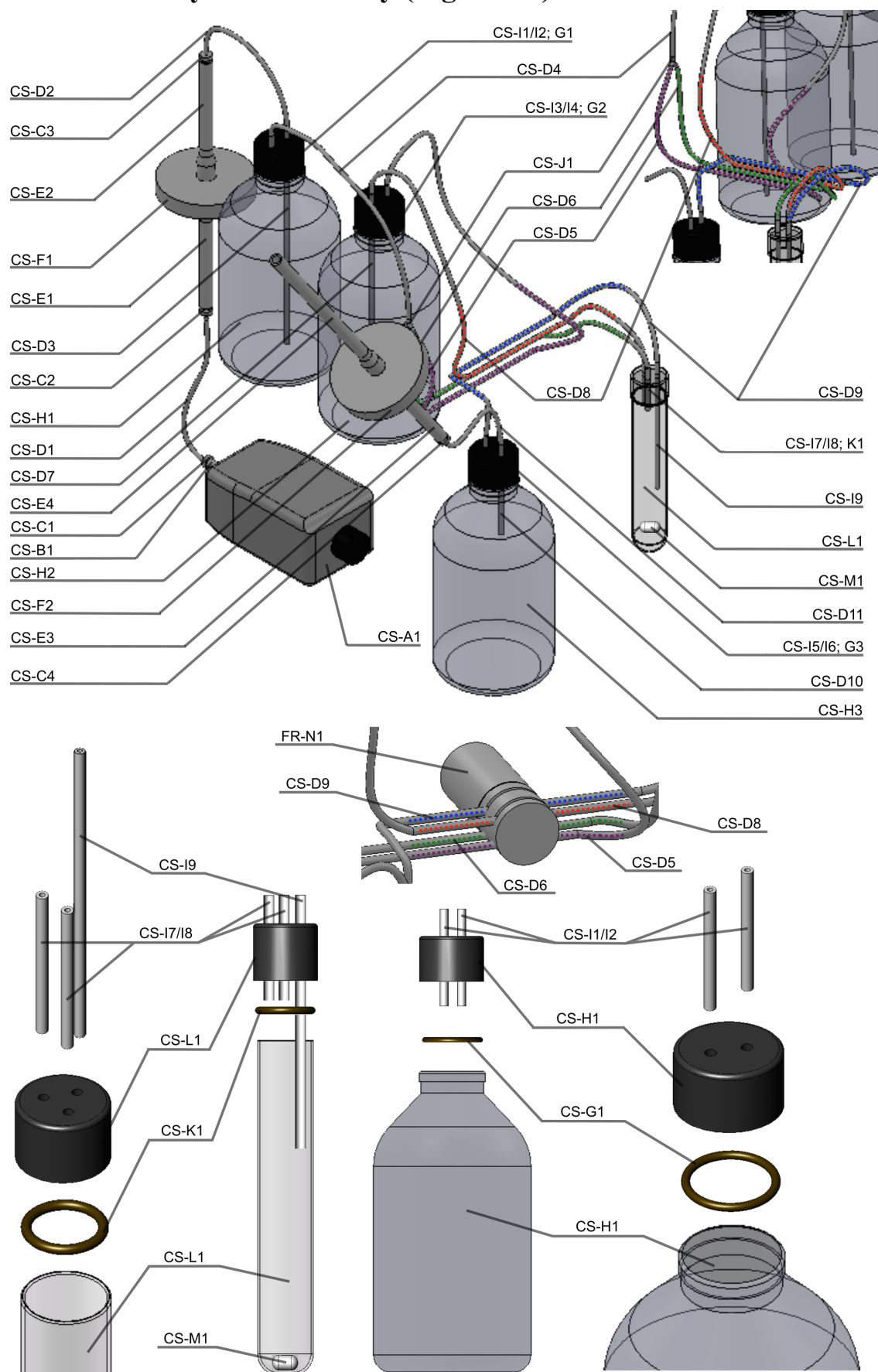
Figure 2 - Culture system assembly (Figure S2)
