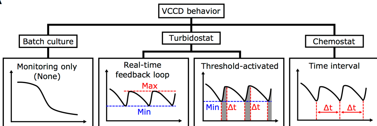
Figure 10 - Illustration of available continuous culture modes (A) and Time interval specific options (B) used to maintain cell growth (Figure 4).
