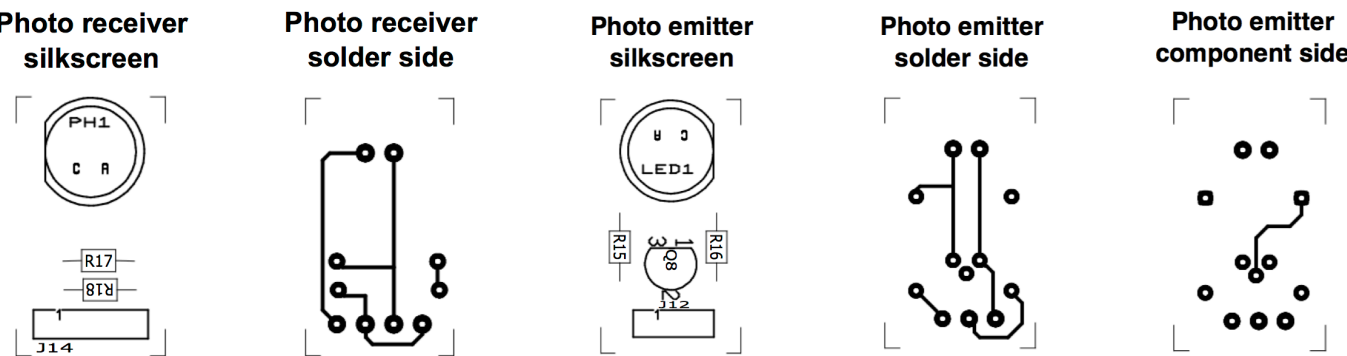
Figure 8 - Details of the photo emitter and receiver PCBs (Figure S8)
